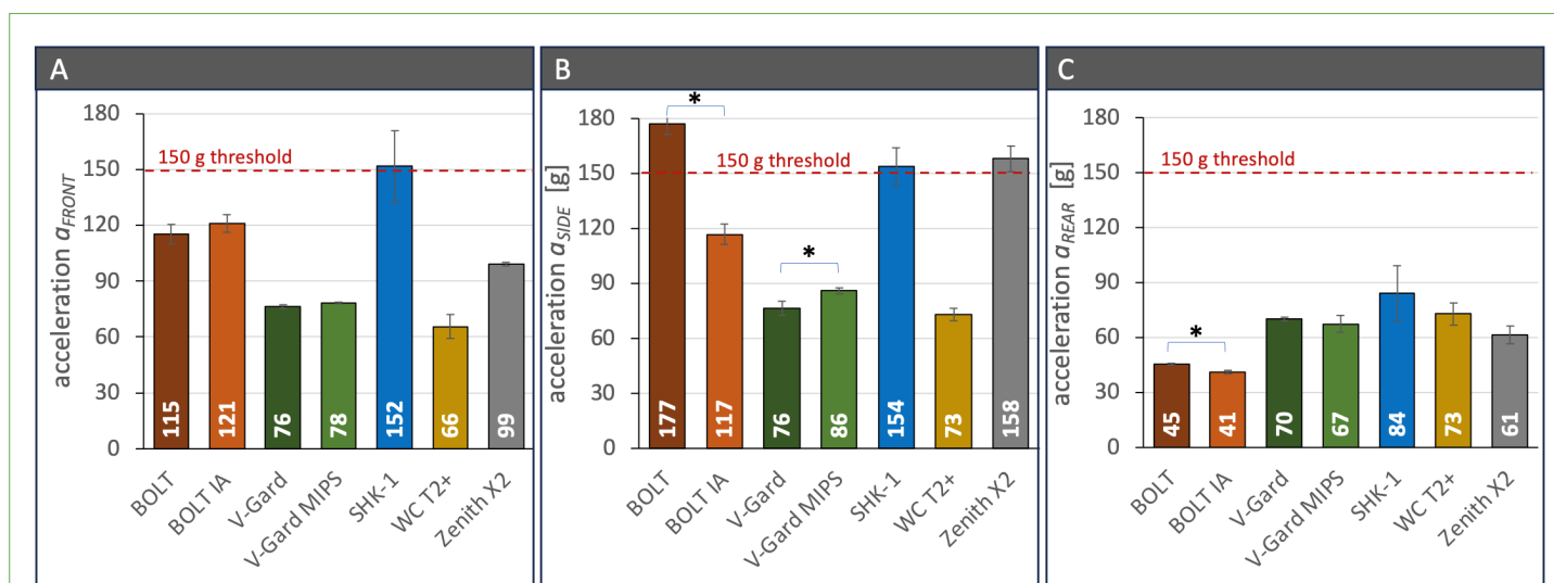
Figure 6: Lateral impact test results, shown for Note: A) Front impacts; B) Side impacts; C) Rear impacts shown in correlation to the 150 g threshold specified in ANSI Z89.1. * indicate significant differences between the same helmet model with and without a rotation-damping technology.
