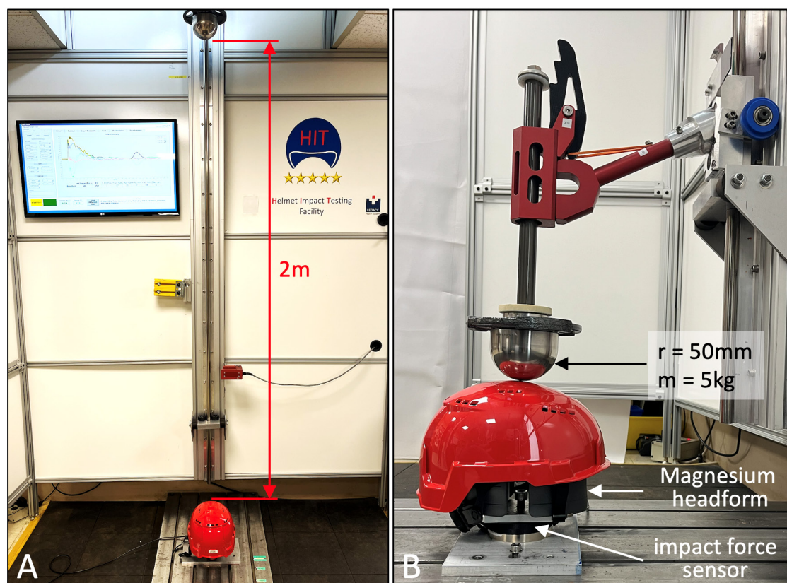
Figure 4: Crown impact testing at 98 J impact energy according to EN 12492. Note: A) A hemispherical impactor is released from 2 m height onto the crown of the helmet; B) The impact force is measured at the base of the headform.
